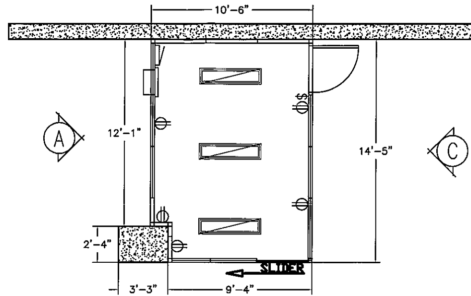
FLOOR PLAN
